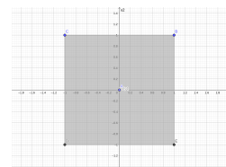
FIGURE 1.2 – B_\infty((0, 0), 1)
