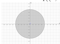
FIGURE 1.1 – B_1((0, 0), 1)
